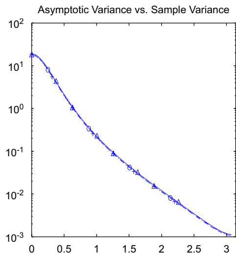
Fig. 1. Example 1. Sample variance (Monte Carlo estimate) vs. normalized frequency ( \omega \in [0, \pi] ). Solid with triangles ( \Delta ): PEM. Dashed with crosses (+): PBSID. Dashed with circles (o): SSARX. Dotted with crosses (+): asymptotic variance for PBSID.
