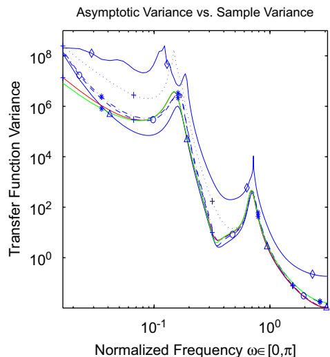
Fig. 5. Asymptotic variance (and its Monte Carlo estimate) Dashed-dotted with circles (○): PBSID opt . Dashed-dotted with stars (*): IEM (Qin & Ljung, 2003b). Dotted with crosses (+): PBSID. Solid with diamonds (◇): Ljung–McKelvey Ljung and McKelvey (1996). Dotted with triangles (Δ): PEM. Solid with stars (green) (*): asymptotic variance for IEM. Dotted with crosses (red) (+): asymptotic variance for PBSID.
